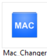
Mac_Changer
